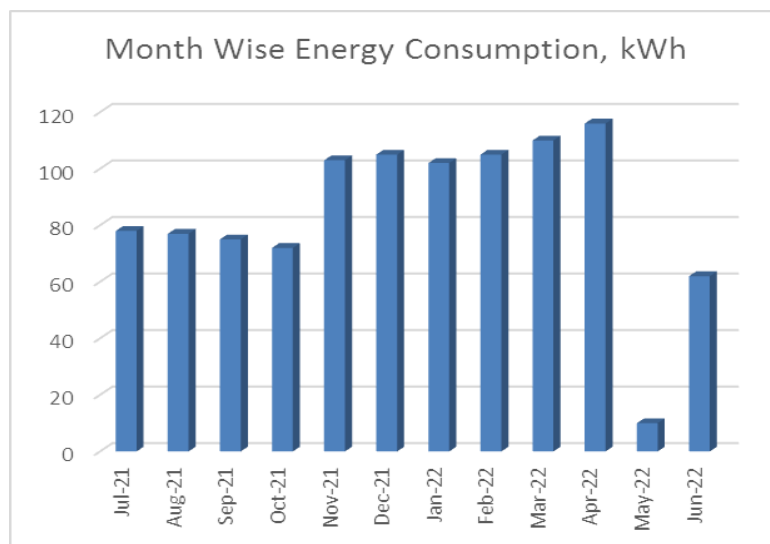
Figure 2.1: Month wise energy consumption
