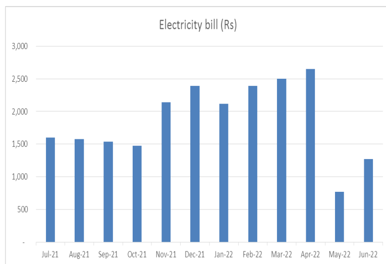
Figure 2.2: Month wise electricity bill
